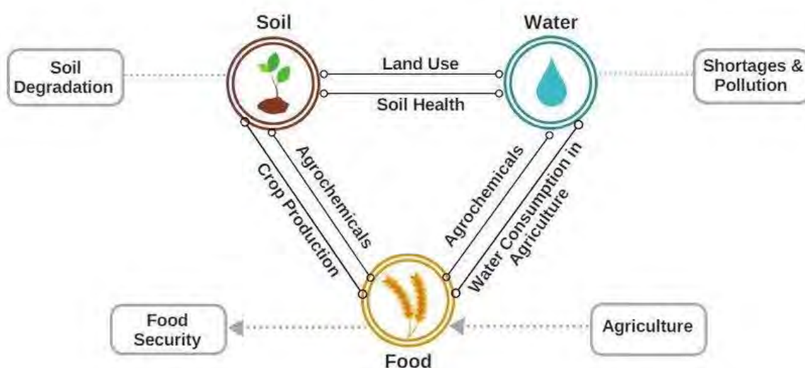
Figure 1. The soil-water nexus relationship
